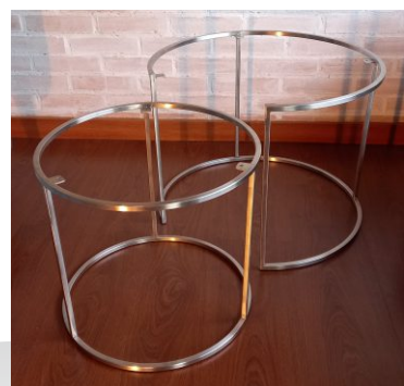
Estructuras especiales para muebles (acero inoxidable y cold rolled) Furniture's special structures (stainless steel and cold rolled)
